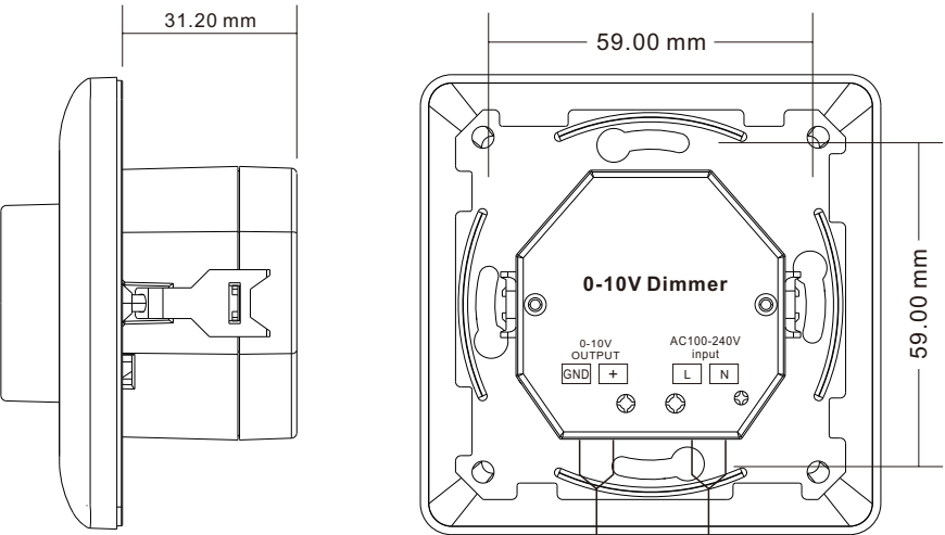
1 channel 1-10V output
