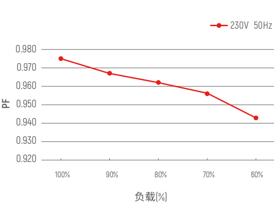
PF vs 负载曲线
