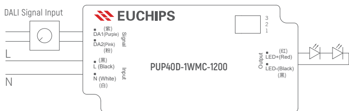
Wiring Diagram
