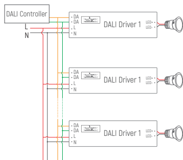
DALI Diagram
