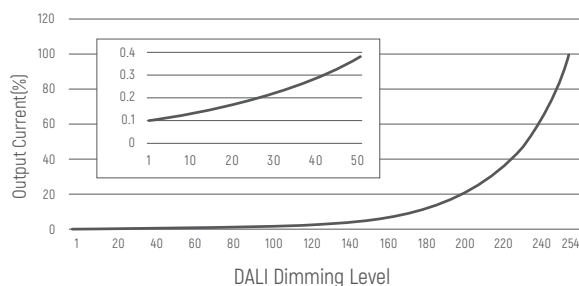
Dimming Curve
