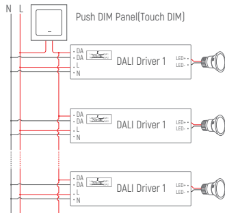
Touch DIM(Push DIM) Diagram
