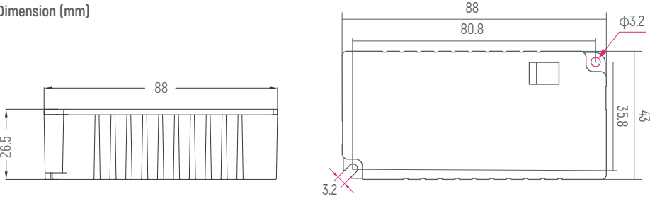
Dimension (mm)
