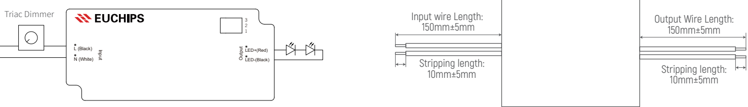
Wiring Diagram
