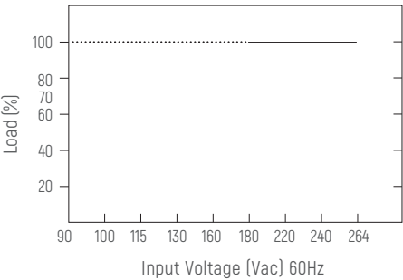
Static characteristic Curve
