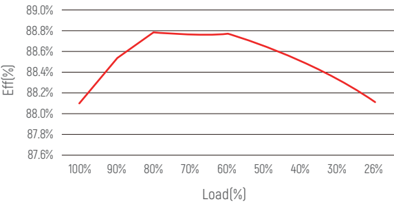
Eff vs load Curve
