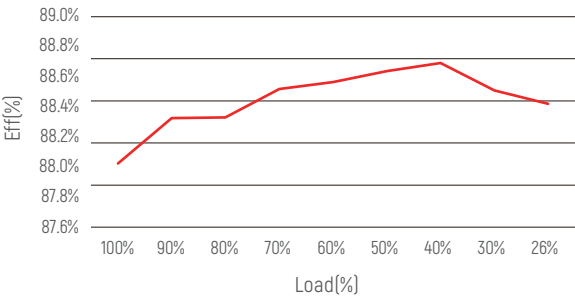
Eff vs load Curve
