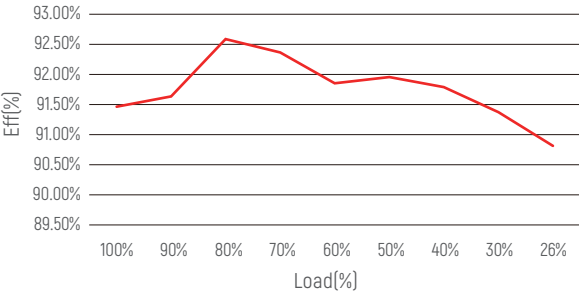
Eff vs load Curve
