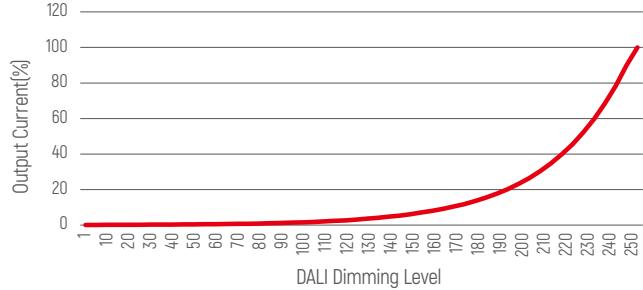
DALI Curve
