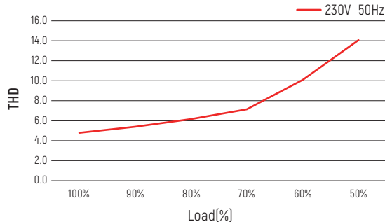
THD vs Load Curve
