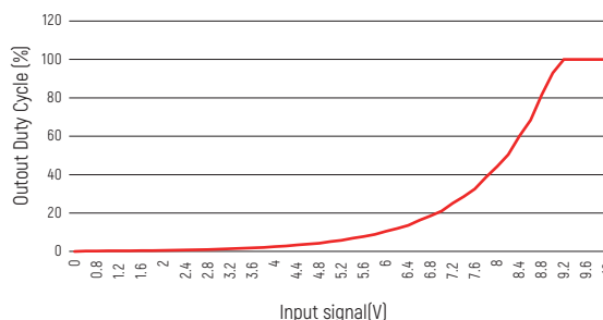
0/1-10V Dimming Curve
