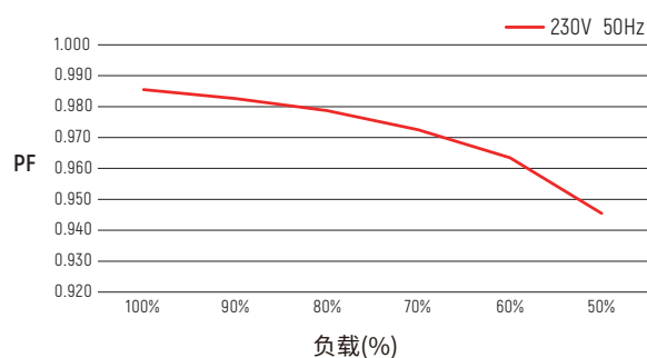
PF vs 负载曲线
