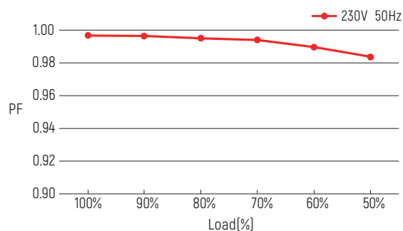
PF vs Load Curve
