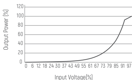
Dimming Curve
