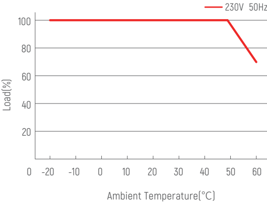
Derating Curve
