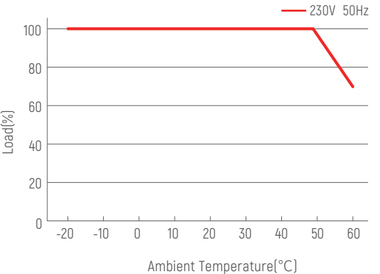
Derating Curve
