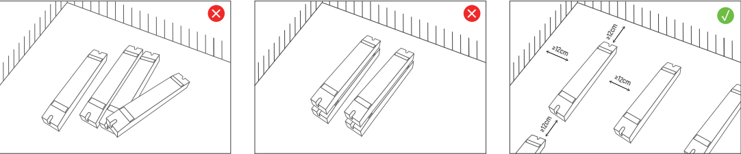
Installation Precautions
