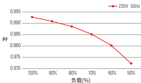
PF vs 负载曲线
