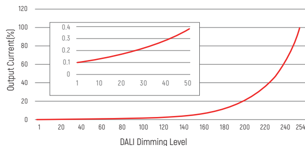
DALI Dimming Curve
