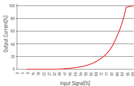
0/1-10V Dimming Curve
