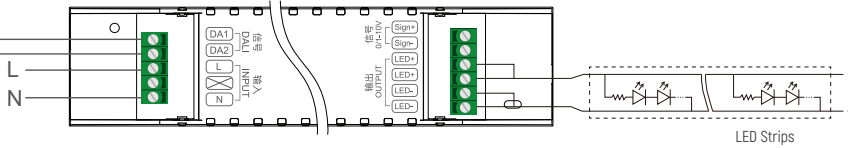
DALI Dimming panel
