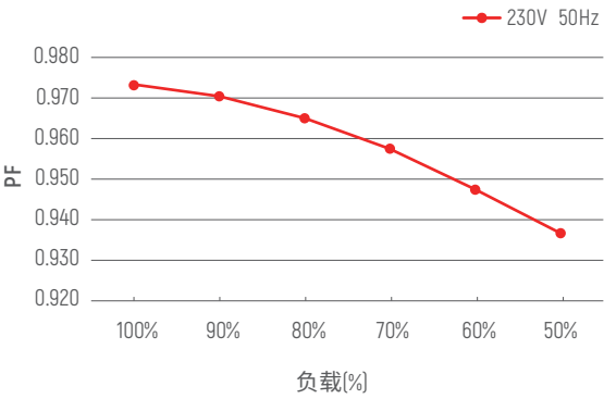
PF vs 负载曲线
