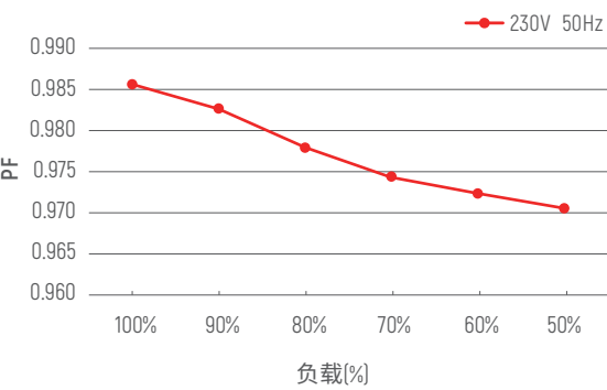
PF vs 负载曲线
