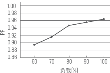
PF VS 负载
