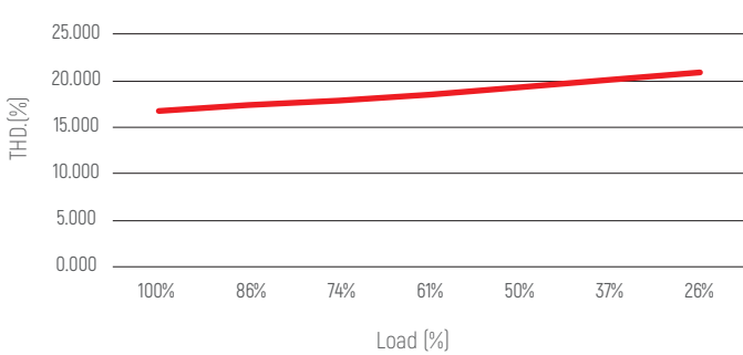
THD vs Load Curve
