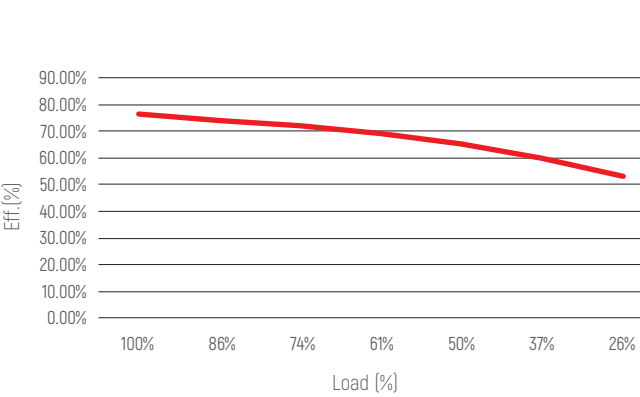
Efficiency vs Load Curve
