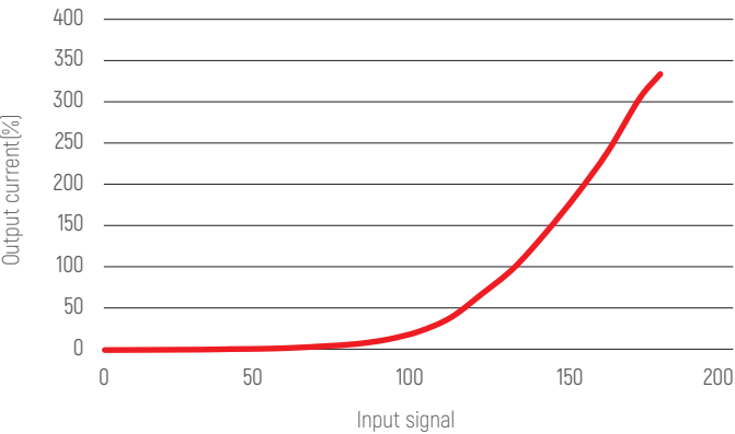
Dimming Curve
