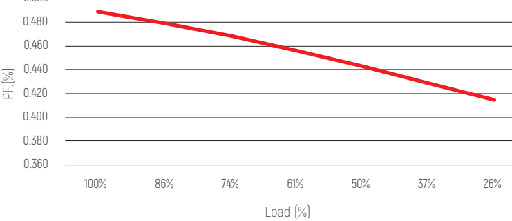
PFvs Load Curve
