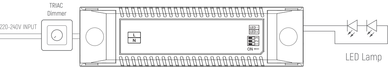
Wiring Diagram
