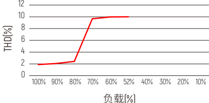
THD曲线
