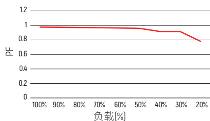
PF vs 负载
