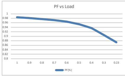
Pf vs load
