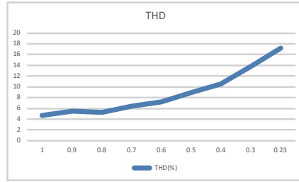
THD
