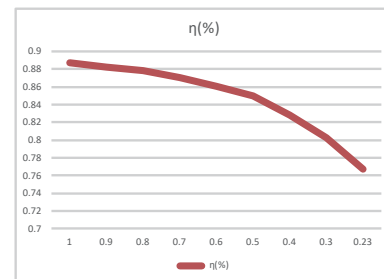
Eff. vs 负载
