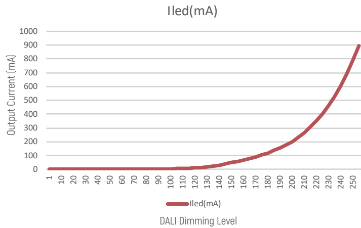
Dimming curve
