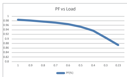
PF vs 负载
