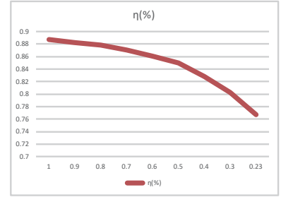
Eff. Vs load
