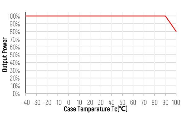
Output Power vs. Case Temperature(Tc)
