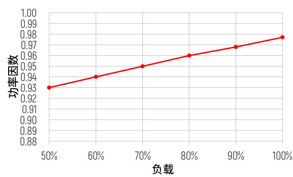
PF vs. 负载
