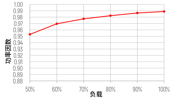
PF vs. 负载
