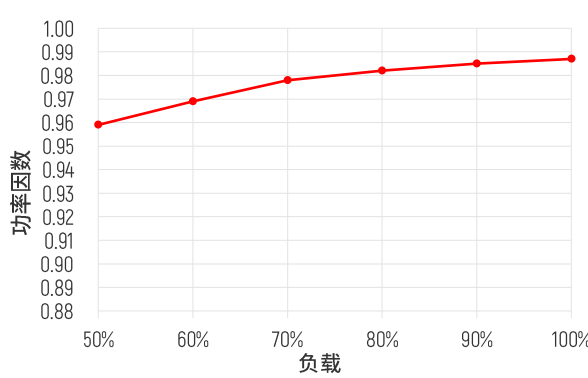
PF vs. 负载
