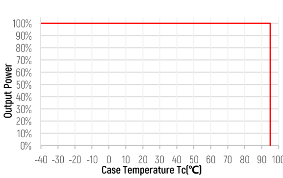
Output Power vs. Case Temperature (Tc)
