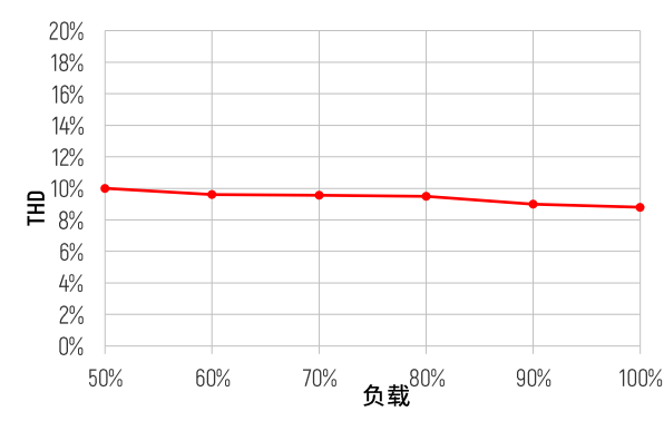
THD vs. 负载
