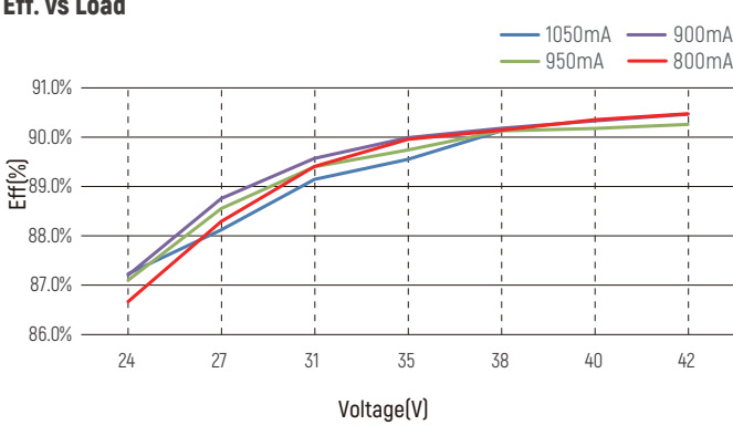
Eff. vs Load
