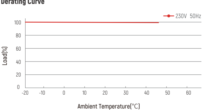
Derating Curve
