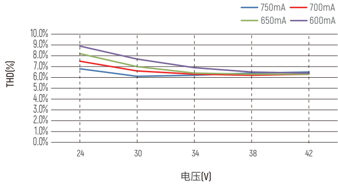
THD vs 负载
