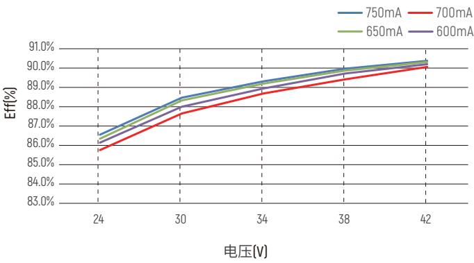
Eff. vs 负载
