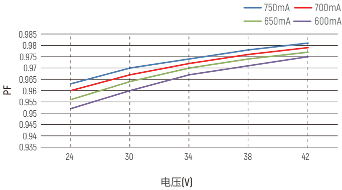
PF vs 负载
