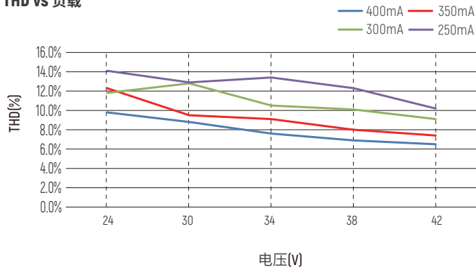
THD vs 负载
