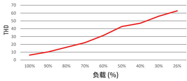
THD曲线
