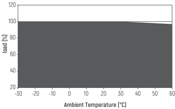
Derating Curve
