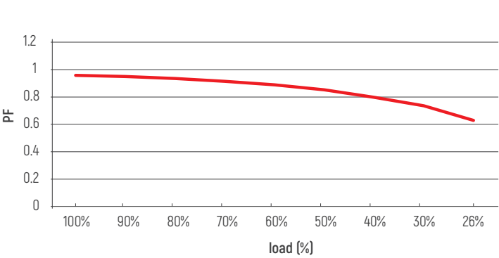
PF Curve
