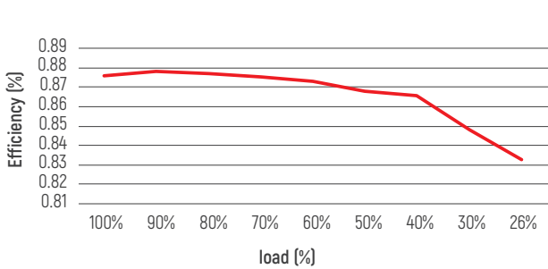
Efficiency Curve
