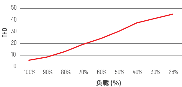
THD曲线
